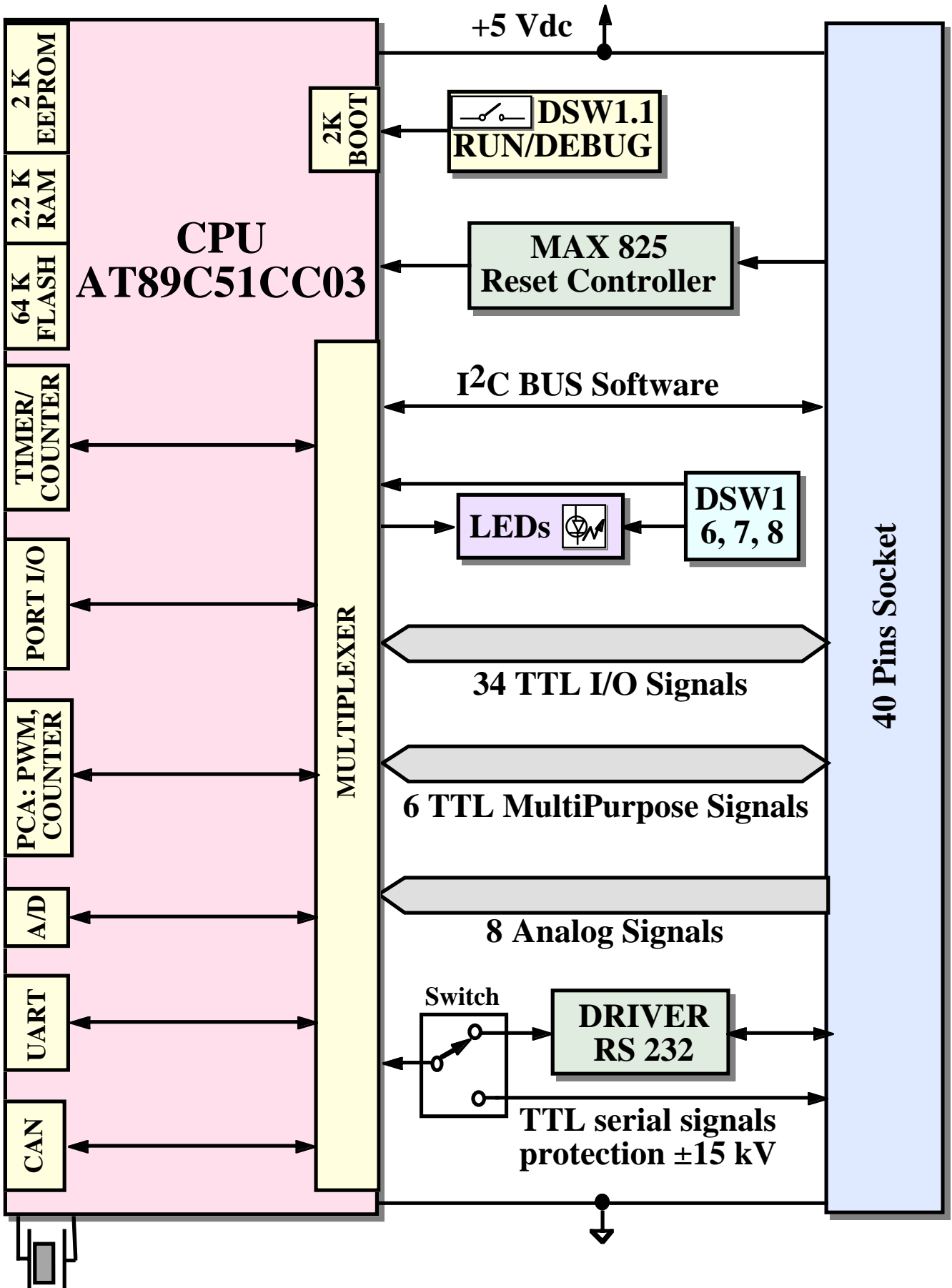
FIGURE 2: BLOCK DIAGRAM
