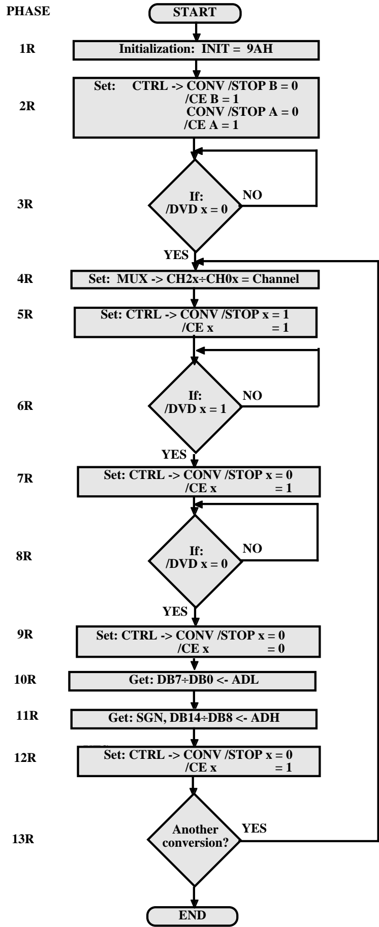
FIGURE 16: SINGLE CONVERSION FLOW CHART
